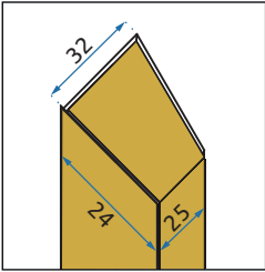
1. Wall-side frame section
