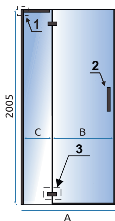
Door (80 cm, 90 cm, 100 cm)
