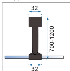
2. Support
