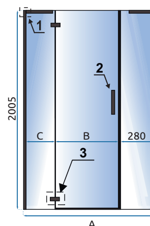
Door + Panel 30 (110 cm, 120 cm, 130 cm)
